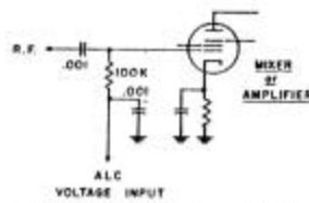
Connecting A.L.C. from the LK-2000 into the Exciter 2309-113
