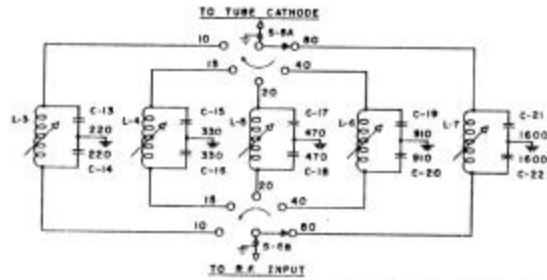
2309-111 Tuned Cathode Input Circuits
