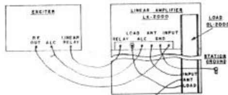
Connections to DL-2000 Dummy Load
