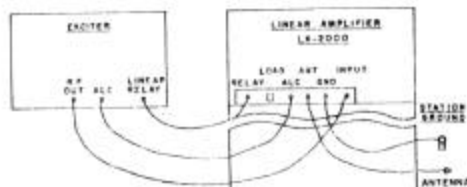
LK-2000 Rear Connections
