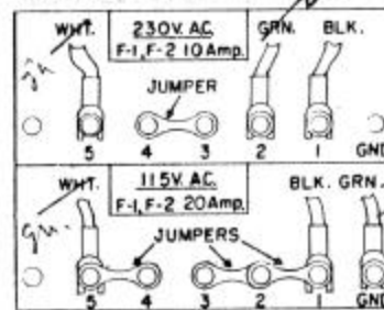
115/230V Line Connections
